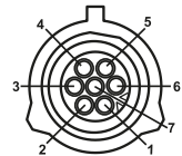
Yan Soketli / Rear Connector
